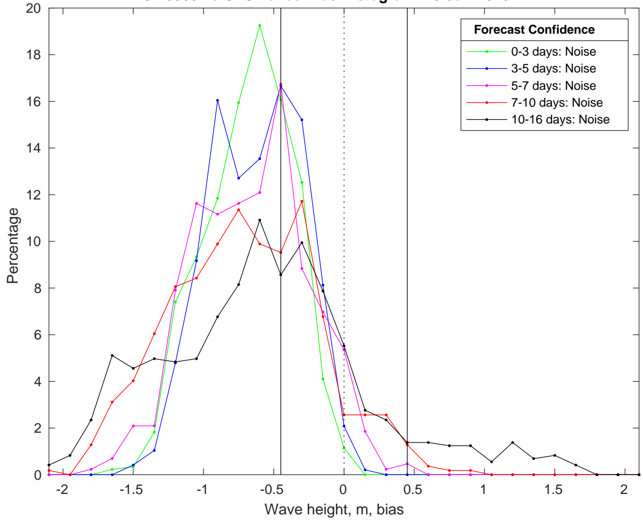
NDBC 46069 vs GFSWaves Bias Histogram: 19-Jan-2025
