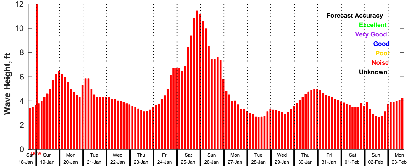
GFS Wave Forecast for NDBC 46069 from 18-Jan-2025 16:00:00 to 03-Feb-2025 16:00:00
