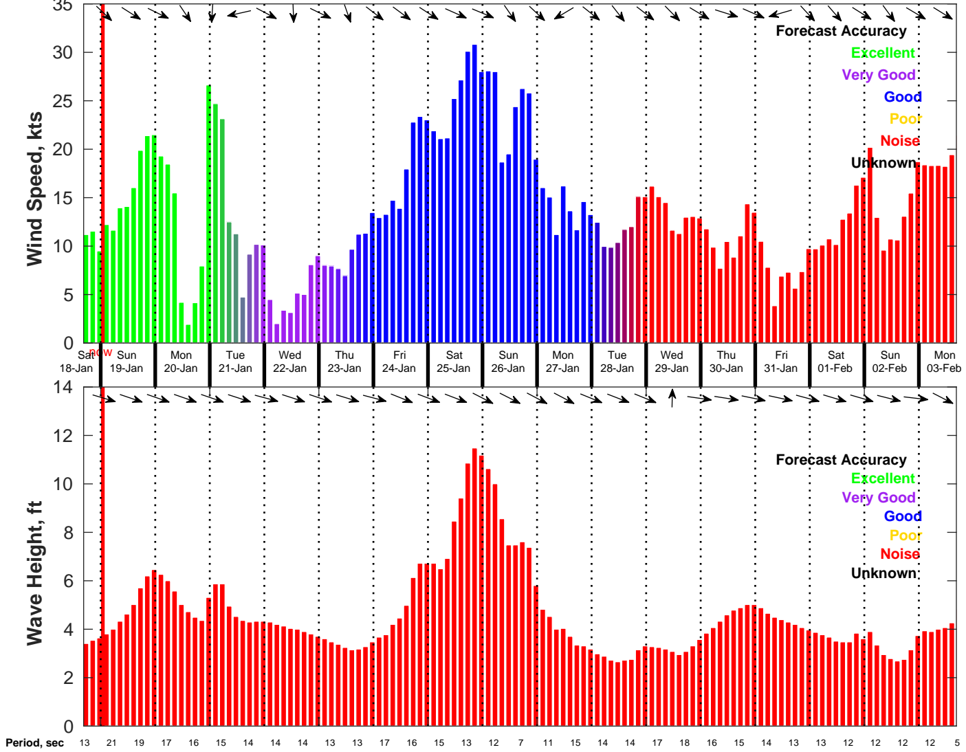
Wind & Wave Forecast for NDBC 46069 from 18-Jan-2025 16:00:00 to 03-Feb-2025 16:00:00
