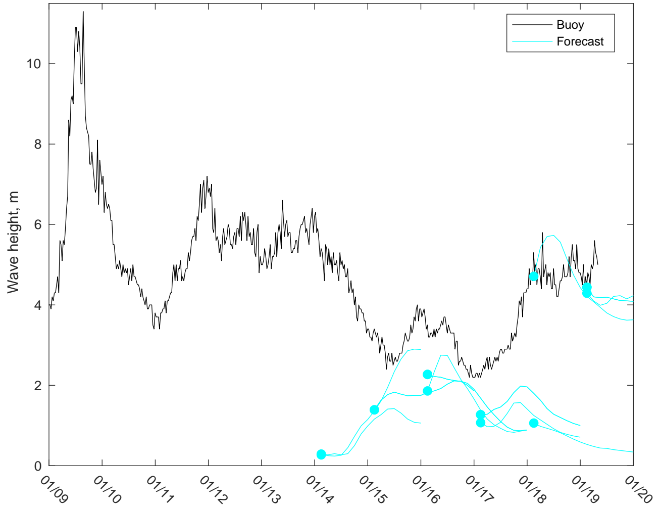
NDBC 46246 vs CMEMSWaves: 5 to 7 day forecast
