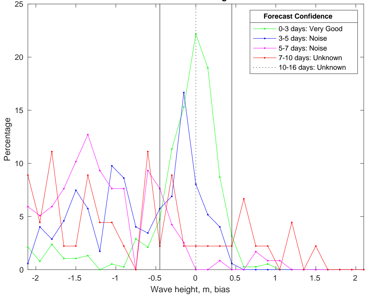
NDBC 46246 vs CMEMSWaves Bias Histogram: 19-Jan-2025
