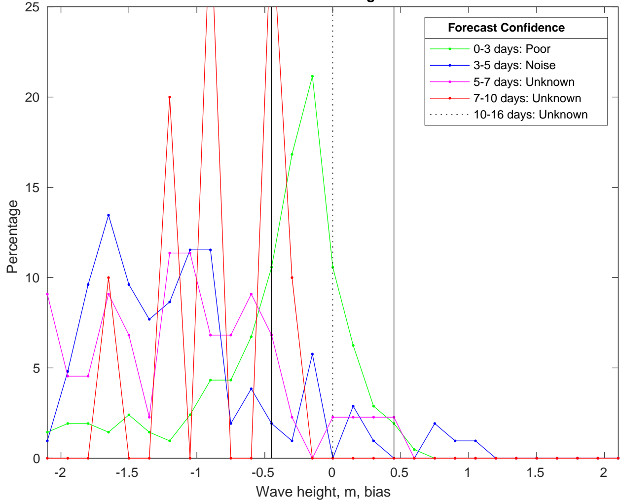
NDBC 46246 vs GFSWaves Bias Histogram: 19-Jan-2025
