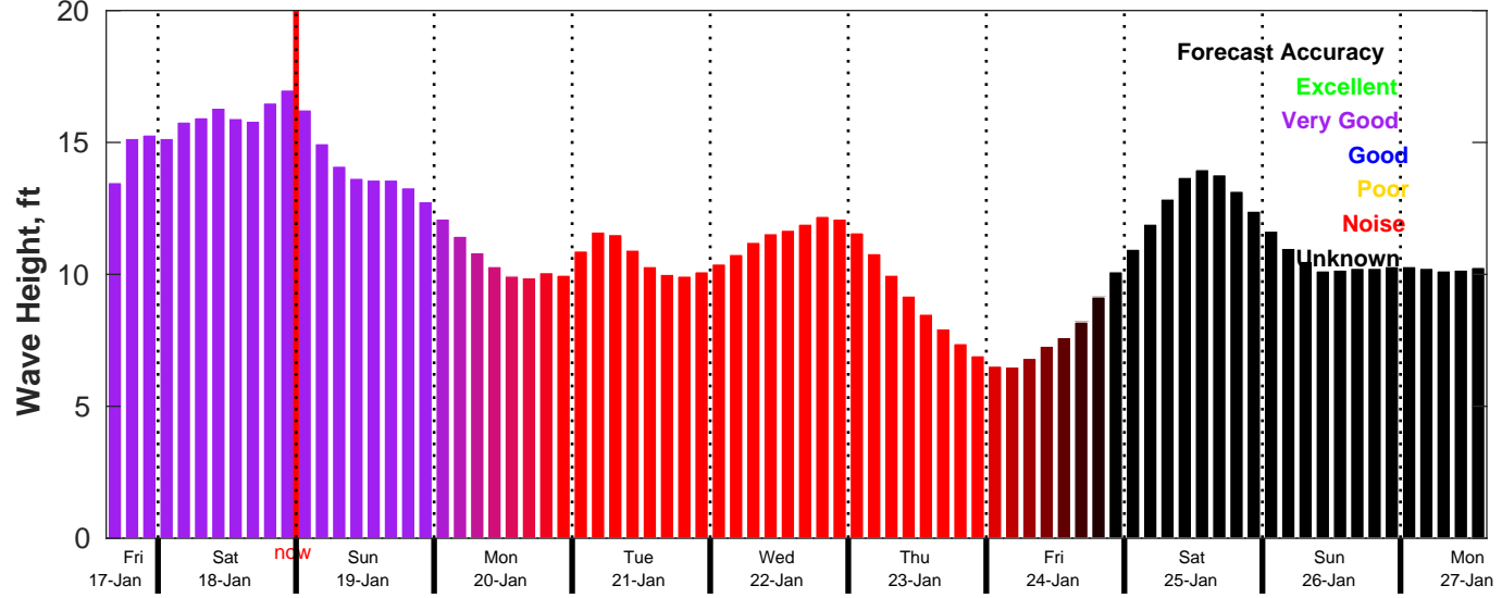
CMEMS Wave Forecast for NDBC 46246 from 17-Jan-2025 15:00:00 to 27-Jan-2025 15:00:00
