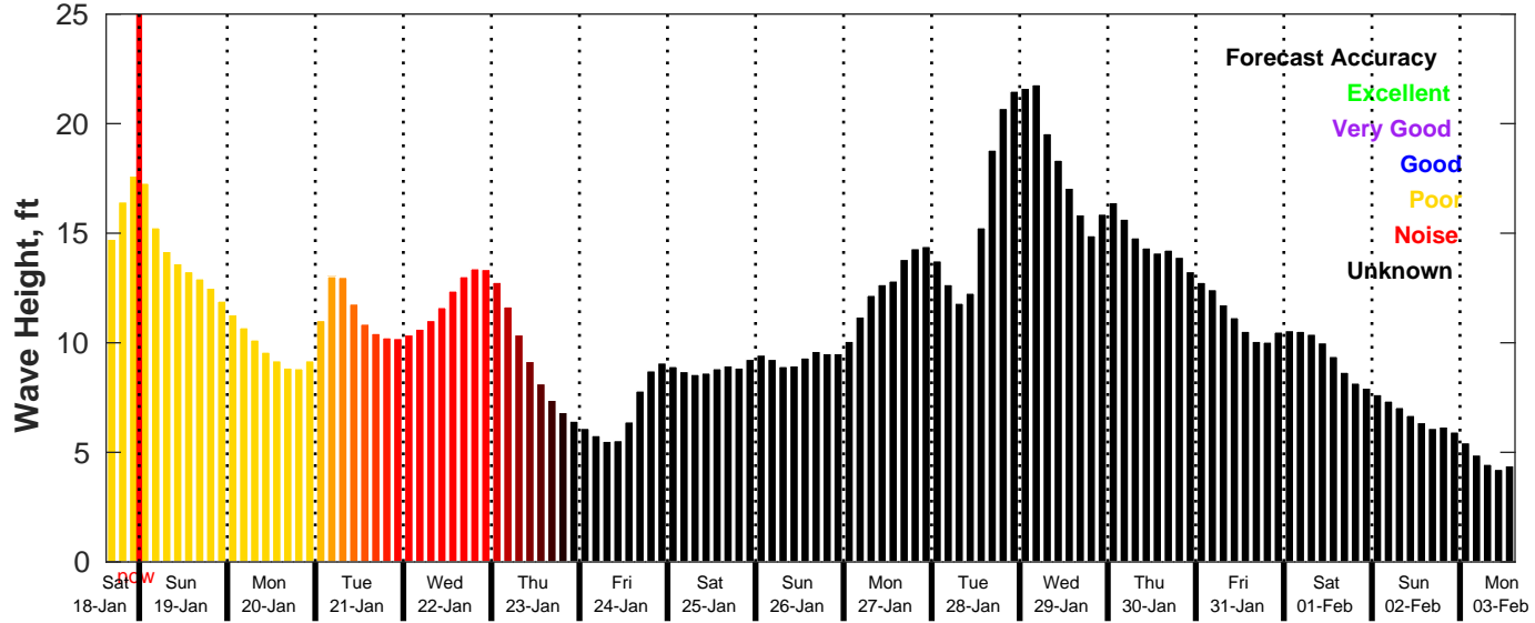
GFS Wave Forecast for NDBC 46246 from 18-Jan-2025 15:00:00 to 03-Feb-2025 15:00:00
