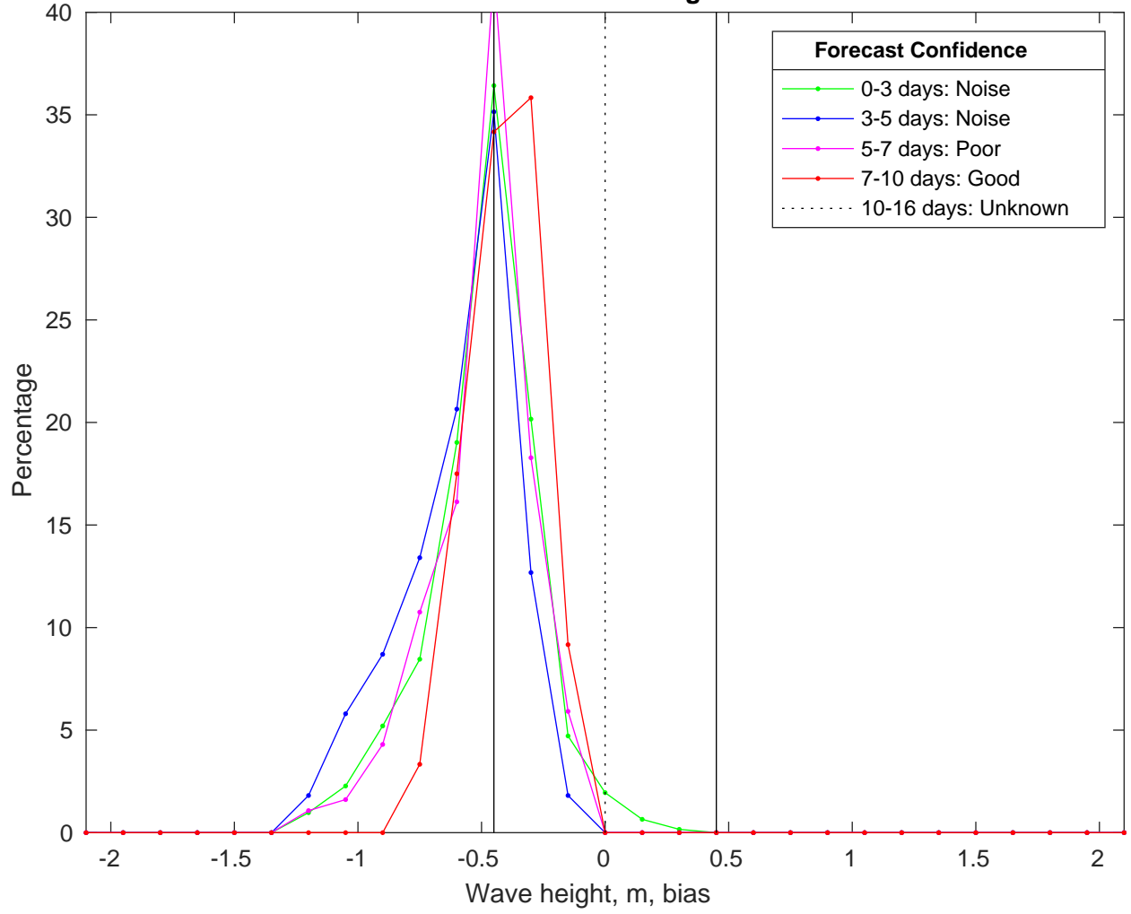
NDBC 51209 vs CMEMSWaves Bias Histogram: 19-Jan-2025
