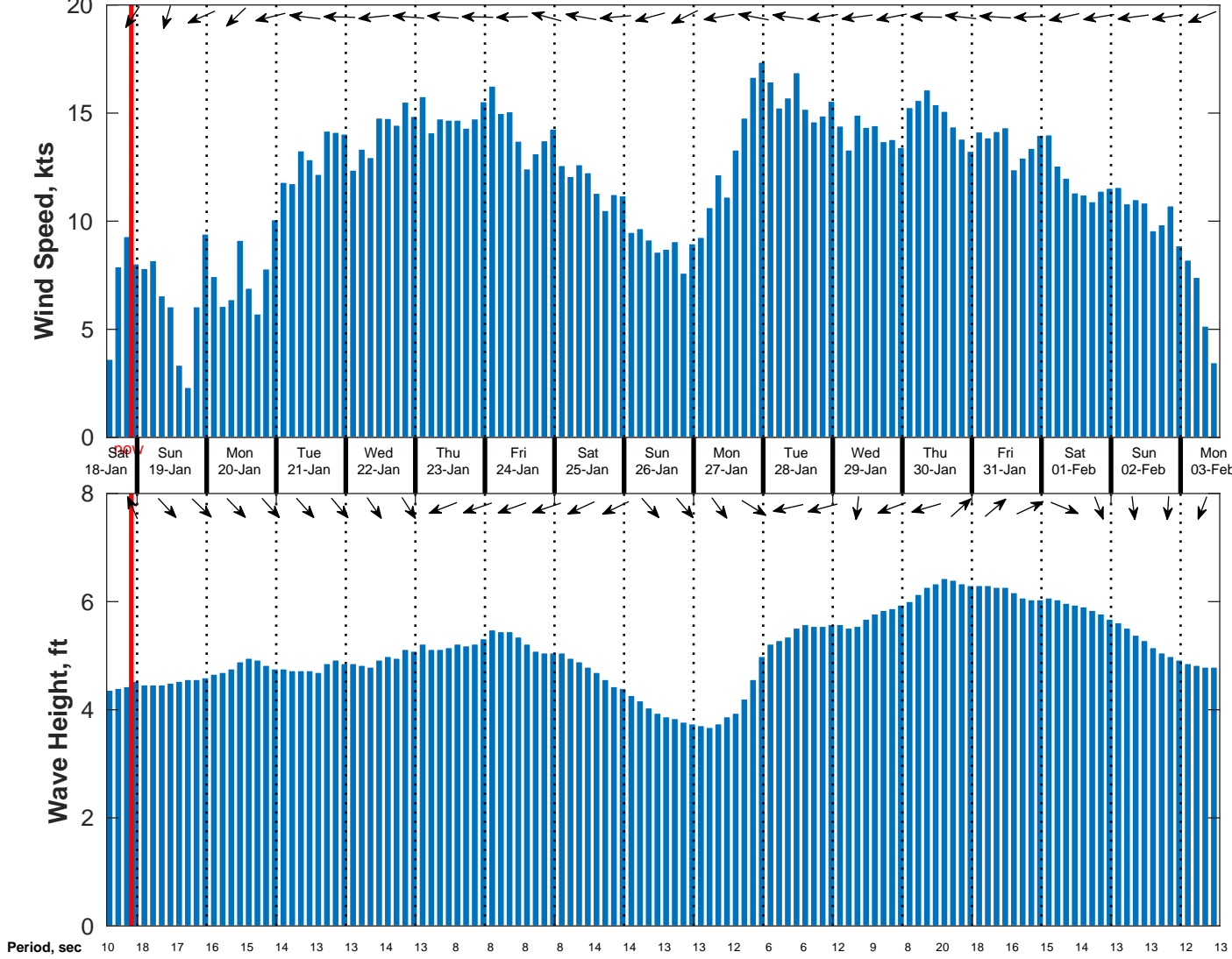
Wind & Wave Forecast for NDBC 51209 from 18-Jan-2025 13:00:00 to 03-Feb-2025 13:00:00
