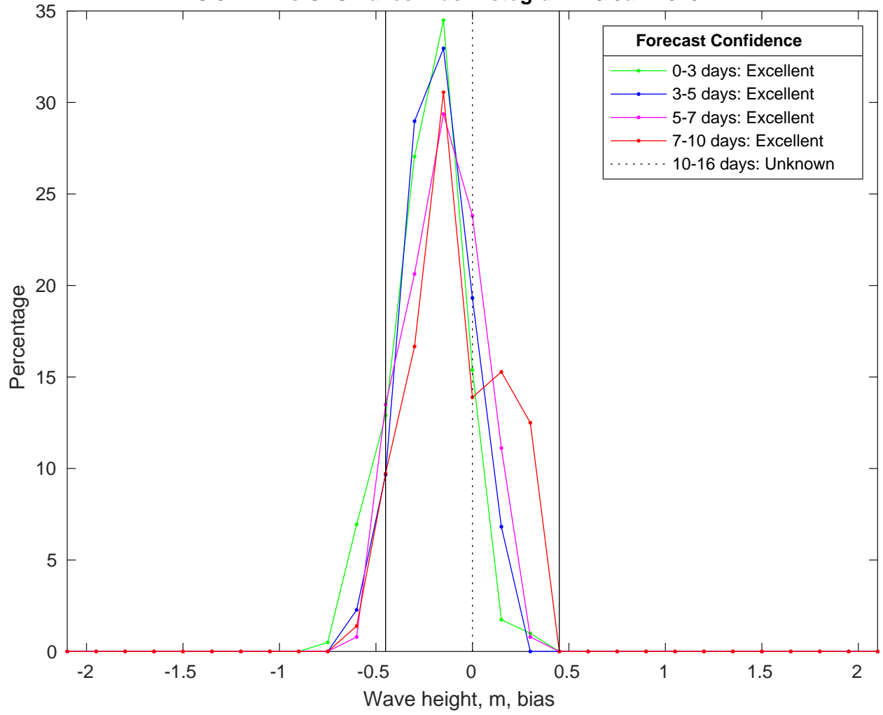
NDBC 52212 vs GFSWaves Bias Histogram: 19-Jan-2025
