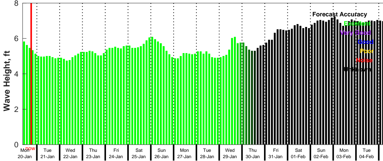
GFS Wave Forecast for NDBC 52212 from 19-Jan-2025 09:00:00 to 04-Feb-2025 09:00:00
