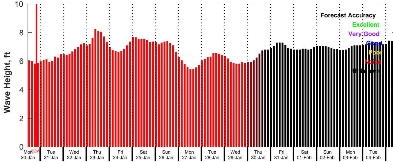
GFS Wave Forecast for NDBC 52213 from 19-Jan-2025 11:00:00 to 04-Feb-2025 11:00:00
