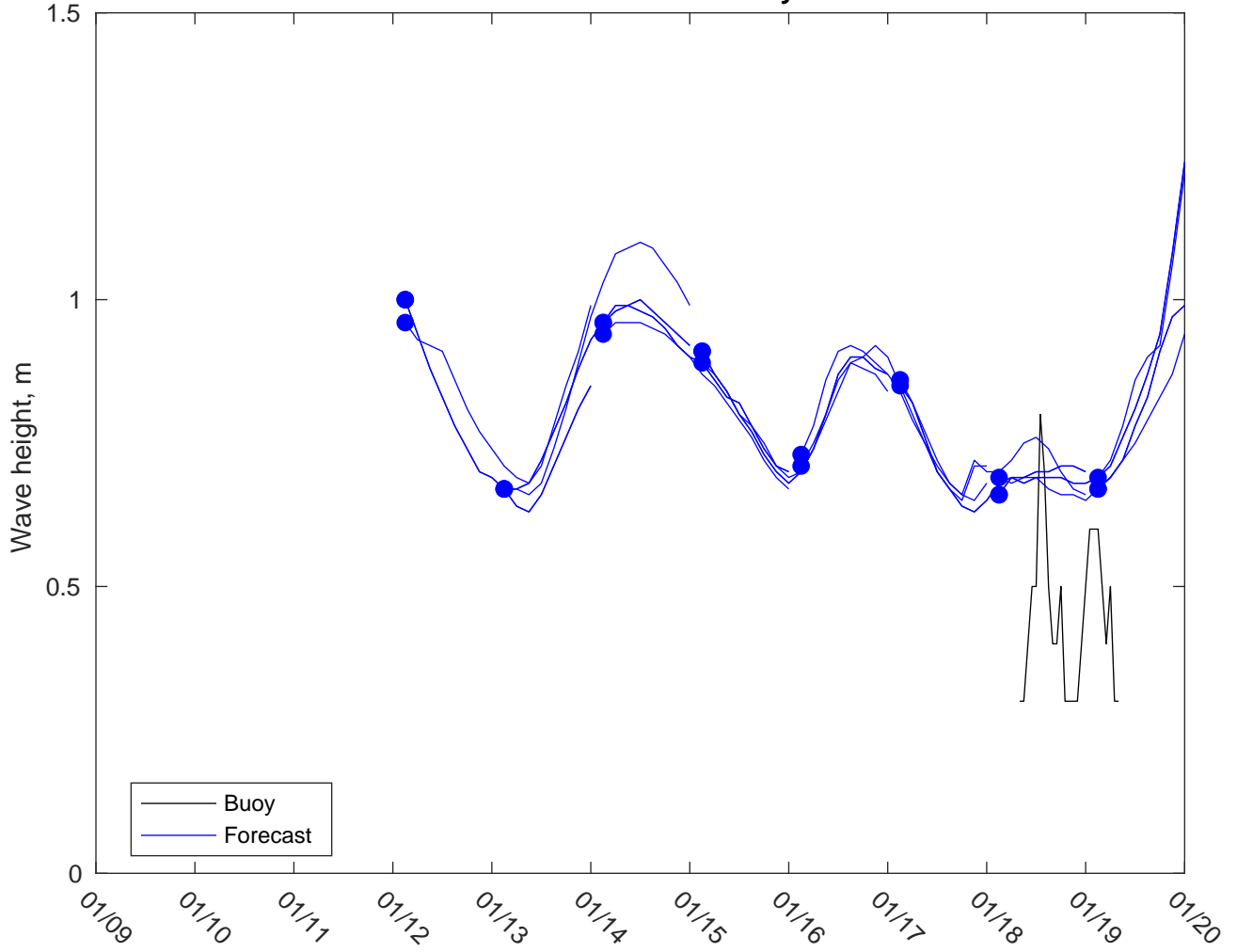
NDBC 62305 vs CMEMSWaves: 3 to 5 day forecast
