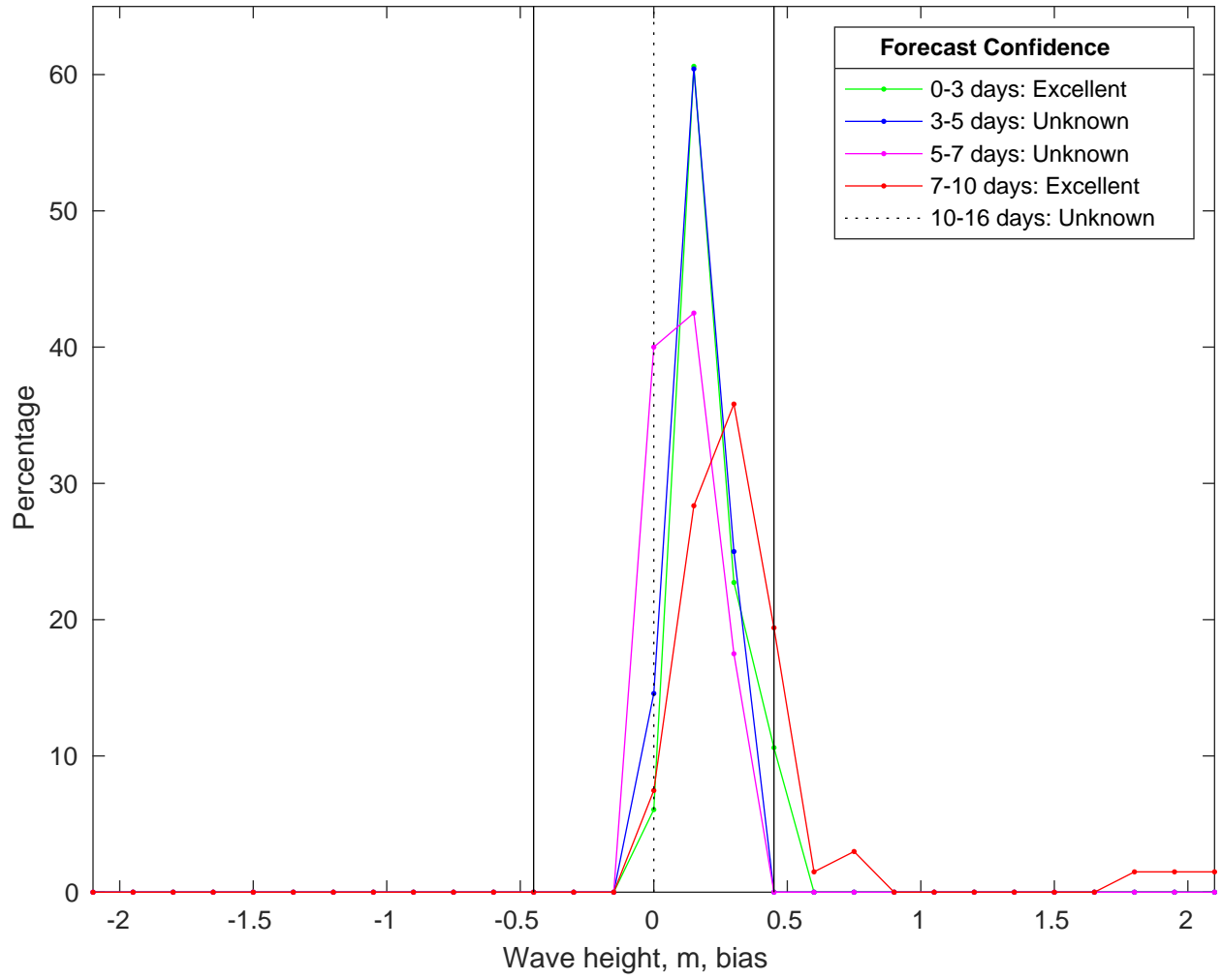
NDBC 62305 vs CMEMSWaves Bias Histogram: 19-Jan-2025
