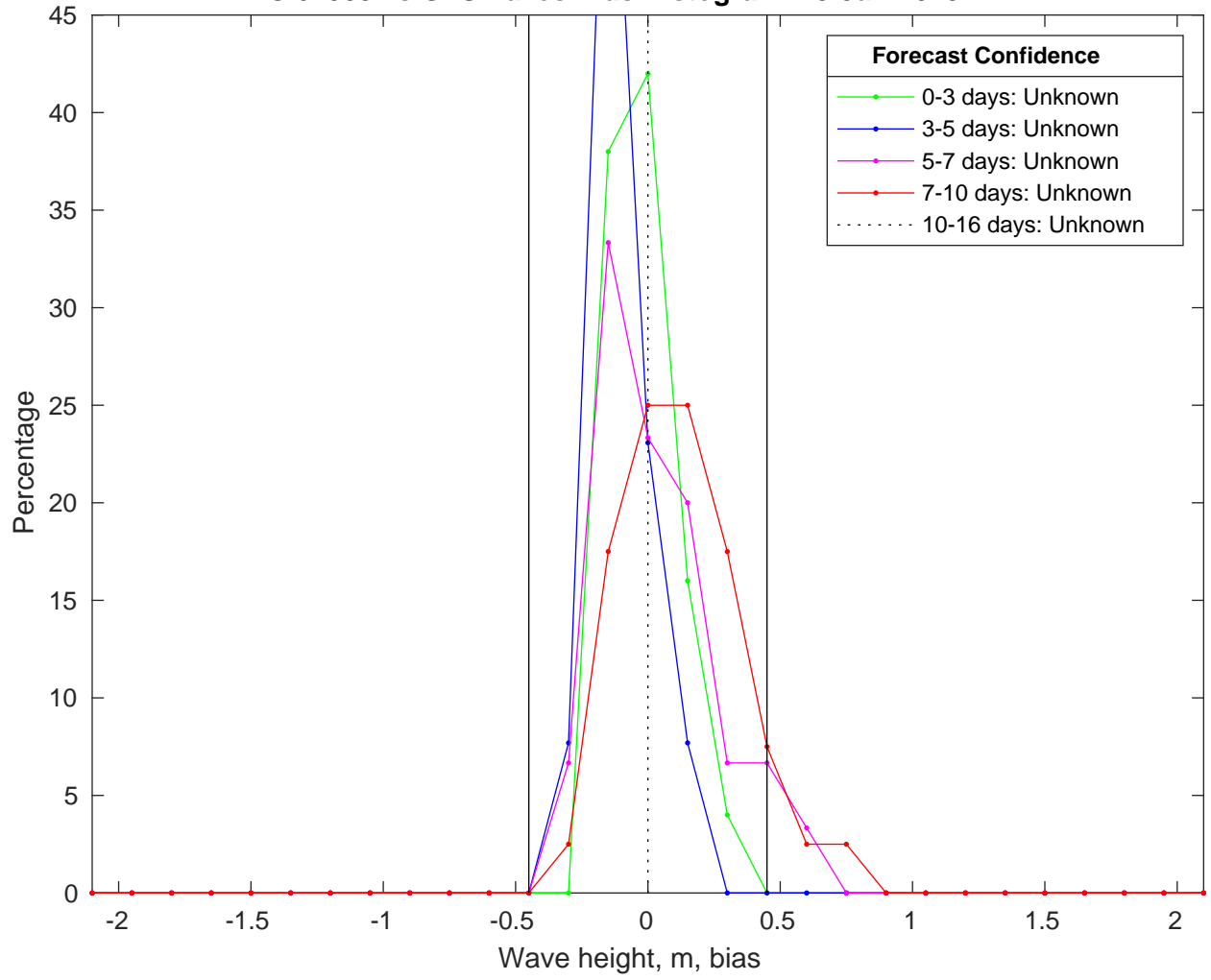
NDBC 62305 vs GFSWaves Bias Histogram: 19-Jan-2025
