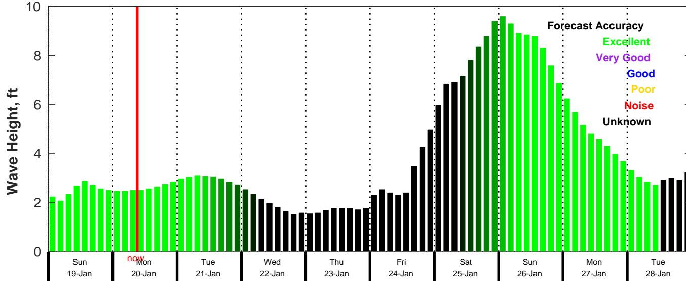
CMEMS Wave Forecast for NDBC 62305 from 18-Jan-2025 00:00:00 to 28-Jan-2025 00:00:00
