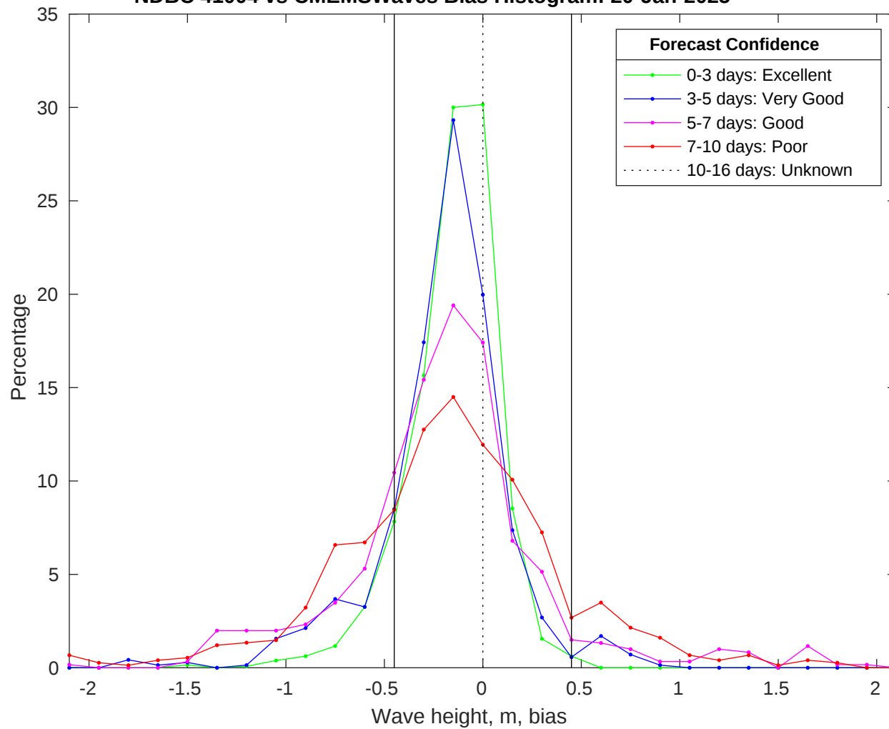
NDBC 41004 vs CMEMSWaves Bias Histogram: 20-Jan-2025
