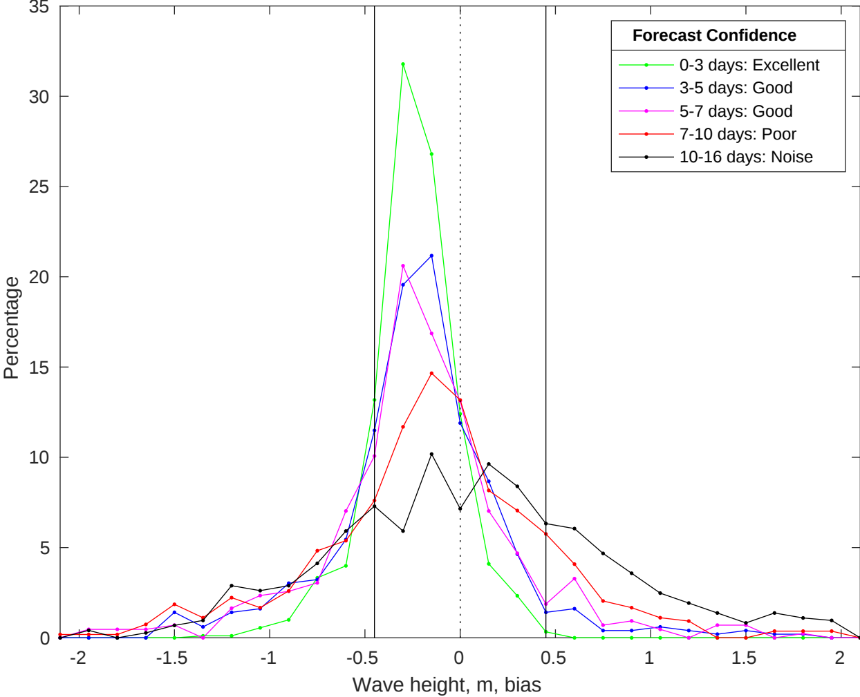
NDBC 41004 vs GFSWaves Bias Histogram: 20-Jan-2025
