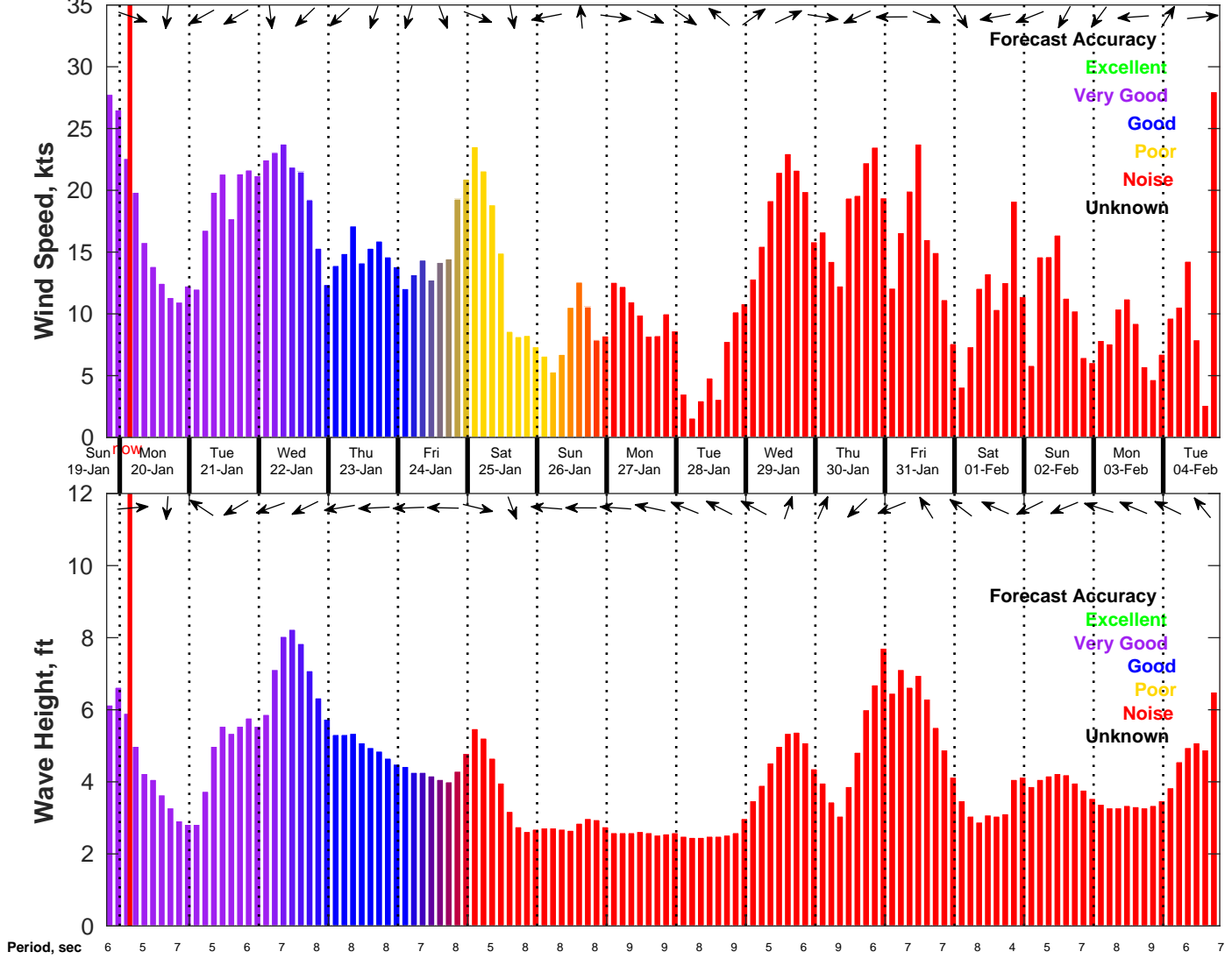
Wind & Wave Forecast for NDBC 41004 from 19-Jan-2025 19:00:00 to 04-Feb-2025 19:00:00
