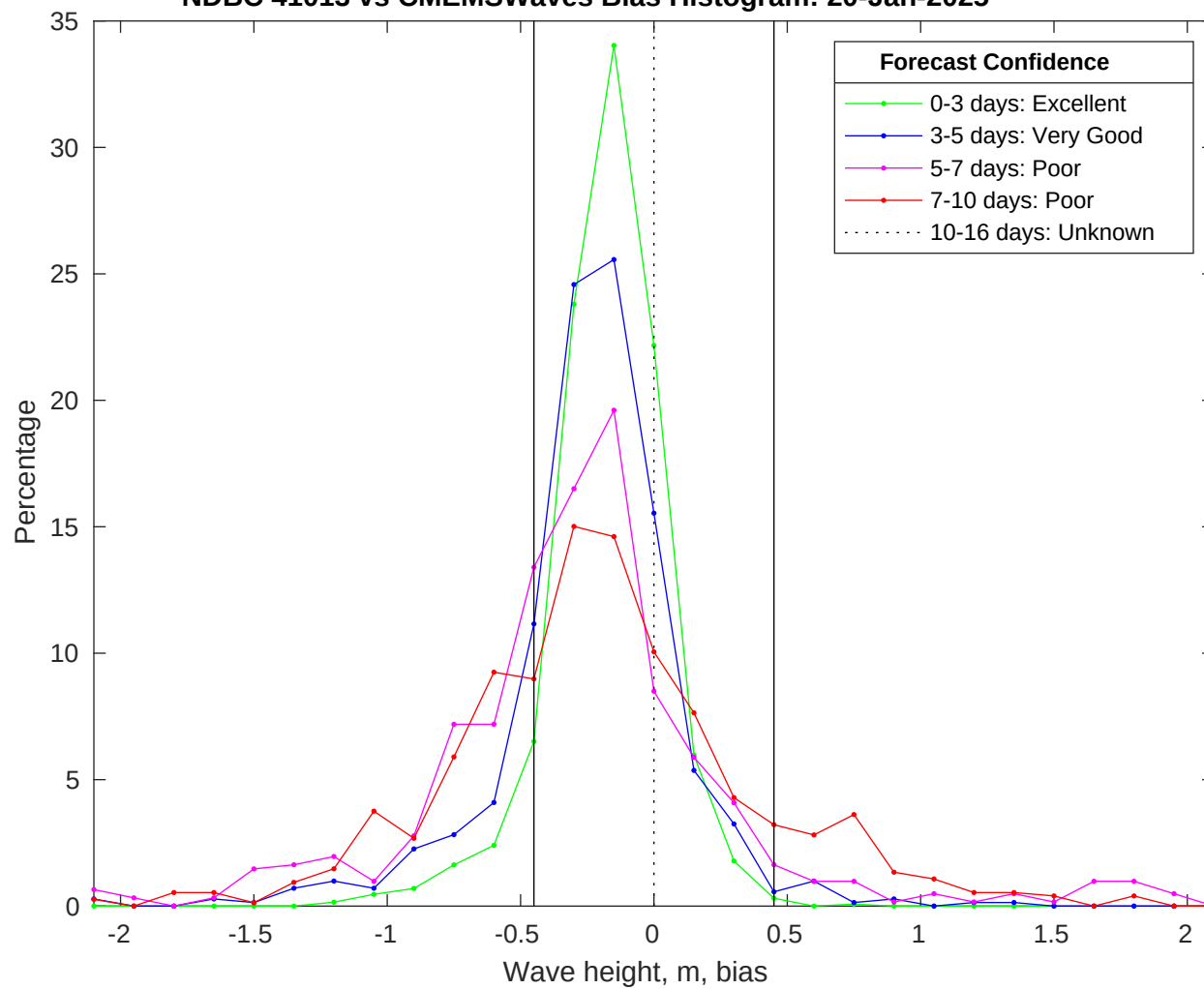
NDBC 41013 vs CMEMSWaves Bias Histogram: 20-Jan-2025
