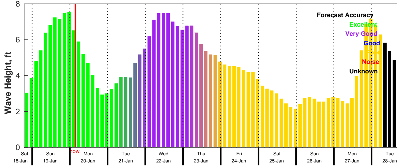
CMEMS Wave Forecast for NDBC 41013 from 18-Jan-2025 19:00:00 to 28-Jan-2025 19:00:00
