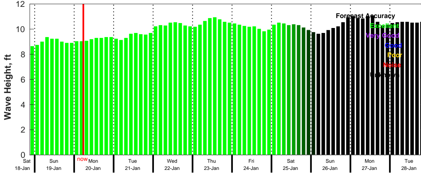
CMEMS Wave Forecast for NDBC 41040 from 18-Jan-2025 21:00:00 to 28-Jan-2025 21:00:00
