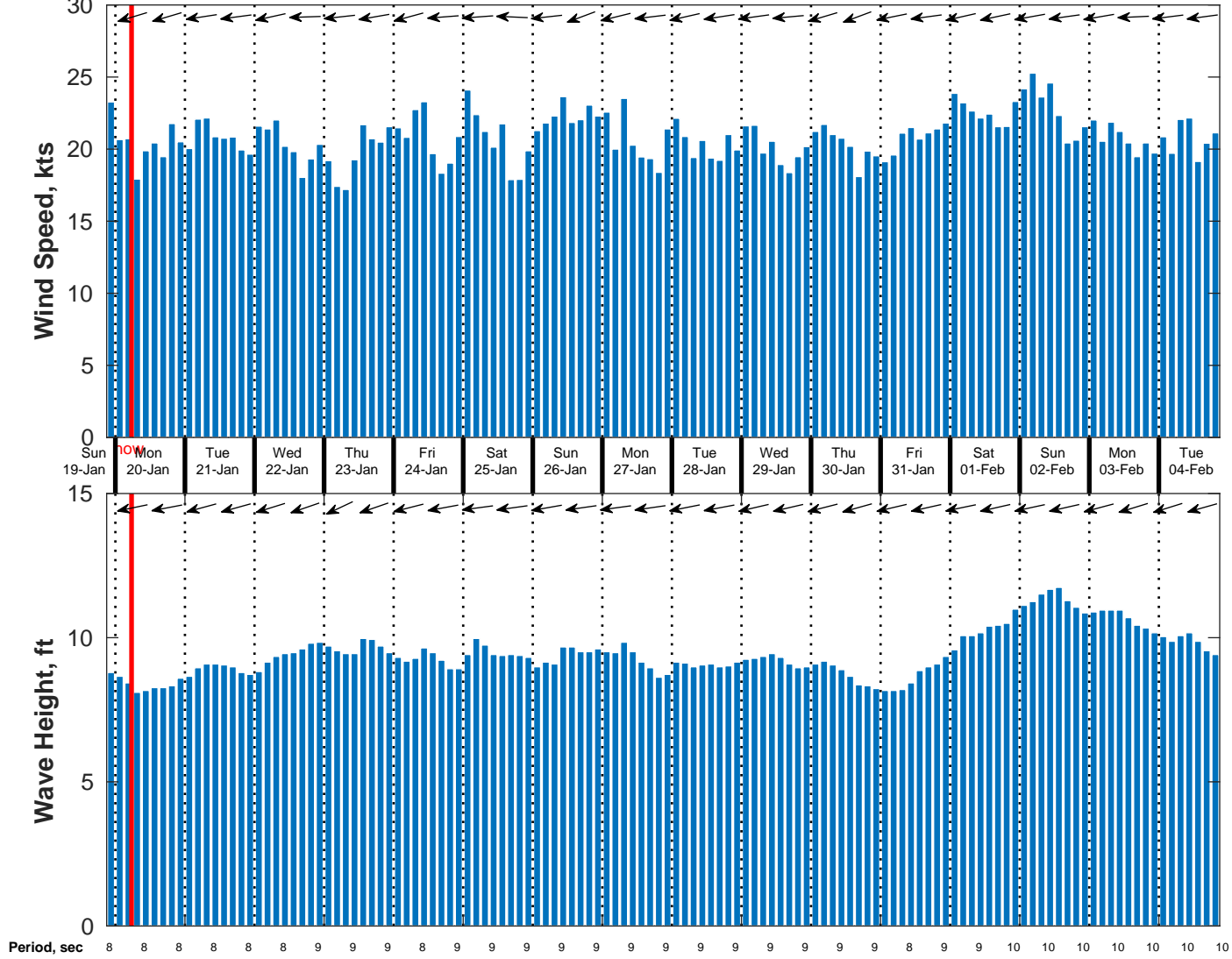
Wind & Wave Forecast for NDBC 41040 from 19-Jan-2025 21:00:00 to 04-Feb-2025 21:00:00
