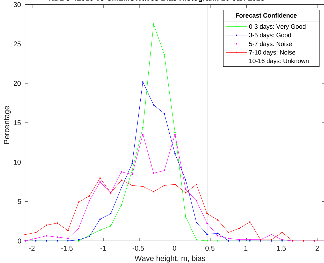
NDBC 42019 vs CMEMSWaves Bias Histogram: 20-Jan-2025
