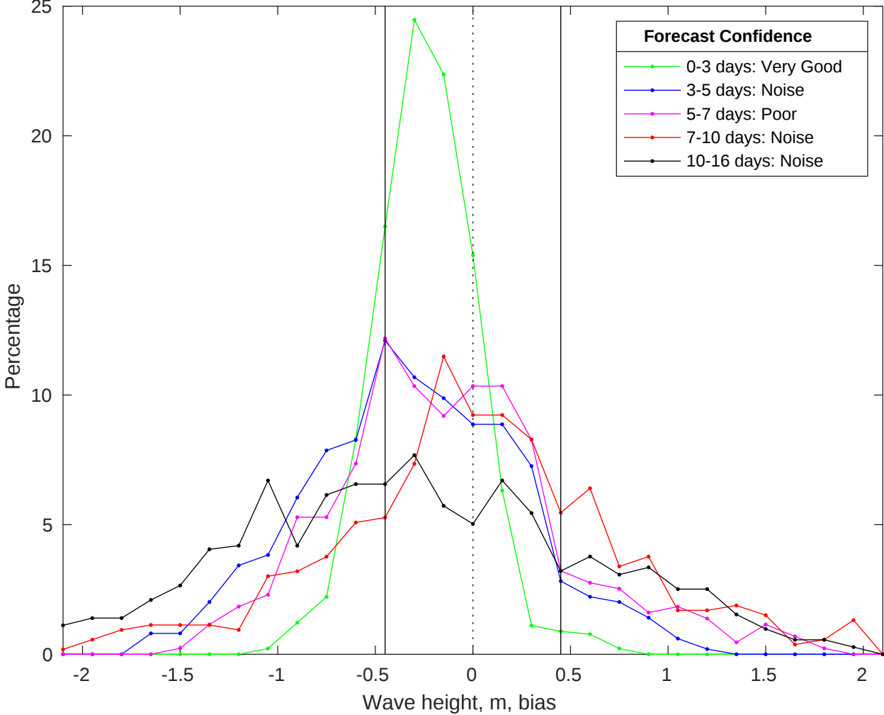
NDBC 42019 vs GFSWaves Bias Histogram: 20-Jan-2025
