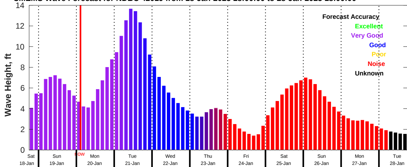
CMEMS Wave Forecast for NDBC 42019 from 18-Jan-2025 18:00:00 to 28-Jan-2025 18:00:00
