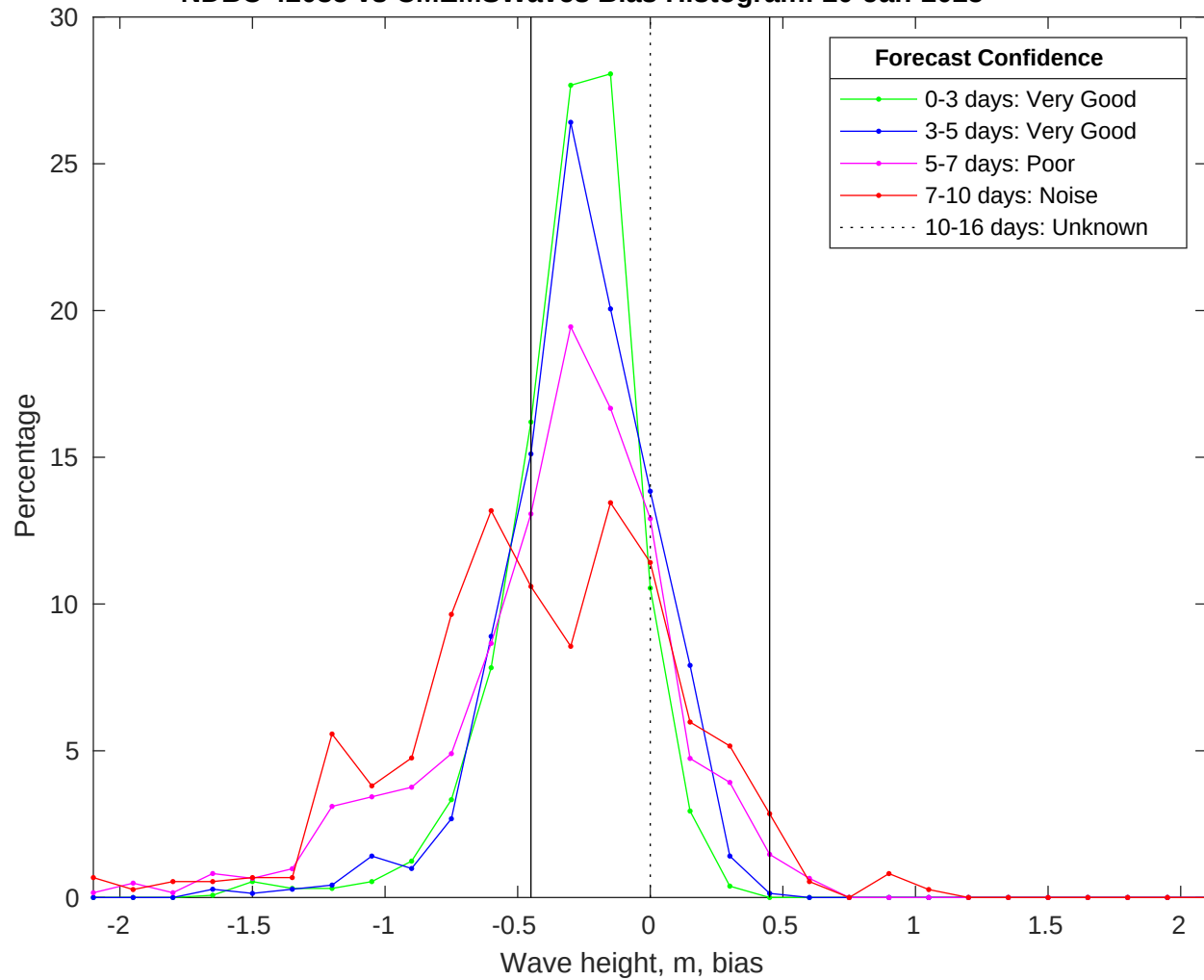
NDBC 42035 vs CMEMSWaves Bias Histogram: 20-Jan-2025
