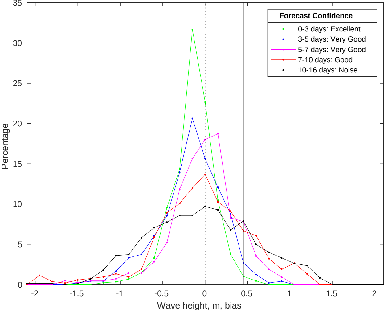
NDBC 42035 vs GFSWaves Bias Histogram: 20-Jan-2025
