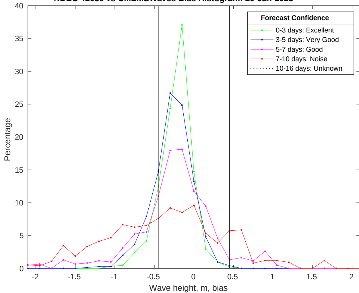
NDBC 42036 vs CMEMSWaves Bias Histogram: 20-Jan-2025
