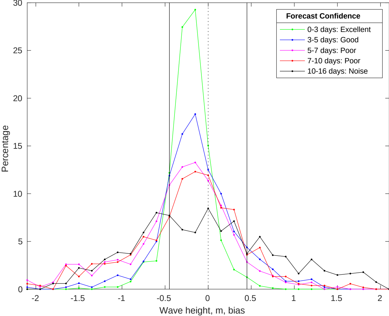
NDBC 42036 vs GFSWaves Bias Histogram: 20-Jan-2025
