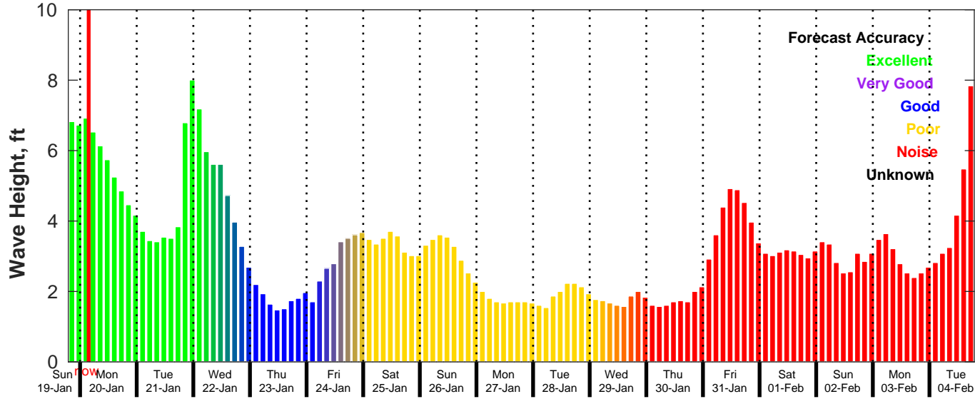
GFS Wave Forecast for NDBC 42036 from 19-Jan-2025 19:00:00 to 04-Feb-2025 19:00:00
