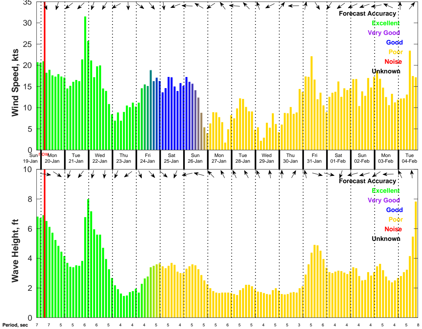
Wind & Wave Forecast for NDBC 42036 from 19-Jan-2025 19:00:00 to 04-Feb-2025 19:00:00
