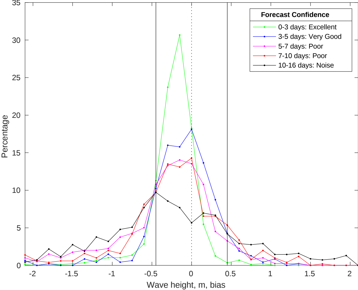
NDBC 42040 vs GFSWaves Bias Histogram: 20-Jan-2025
