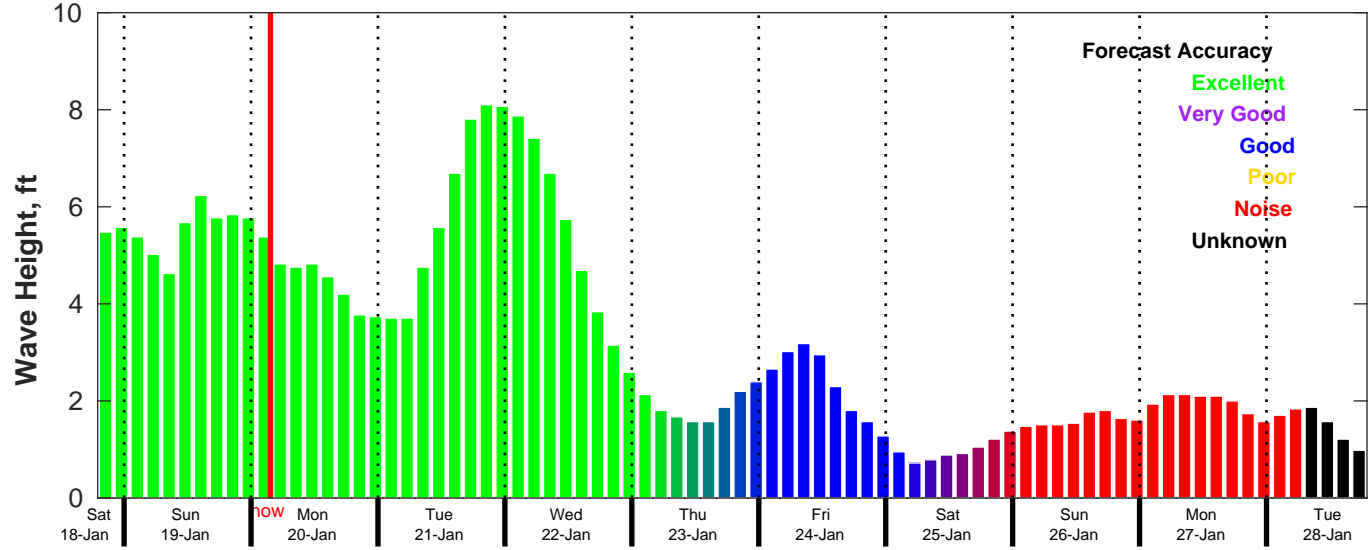
CMEMS Wave Forecast for NDBC 42040 from 18-Jan-2025 19:00:00 to 28-Jan-2025 19:00:00
