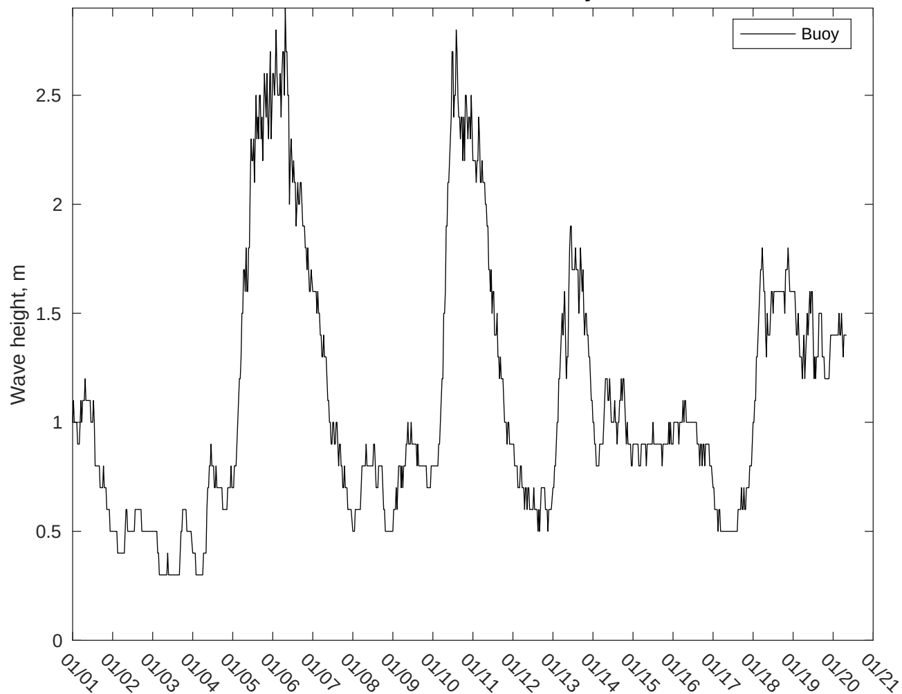
NDBC 42084 vs CMEMSWaves: 10 to 16 day forecast
