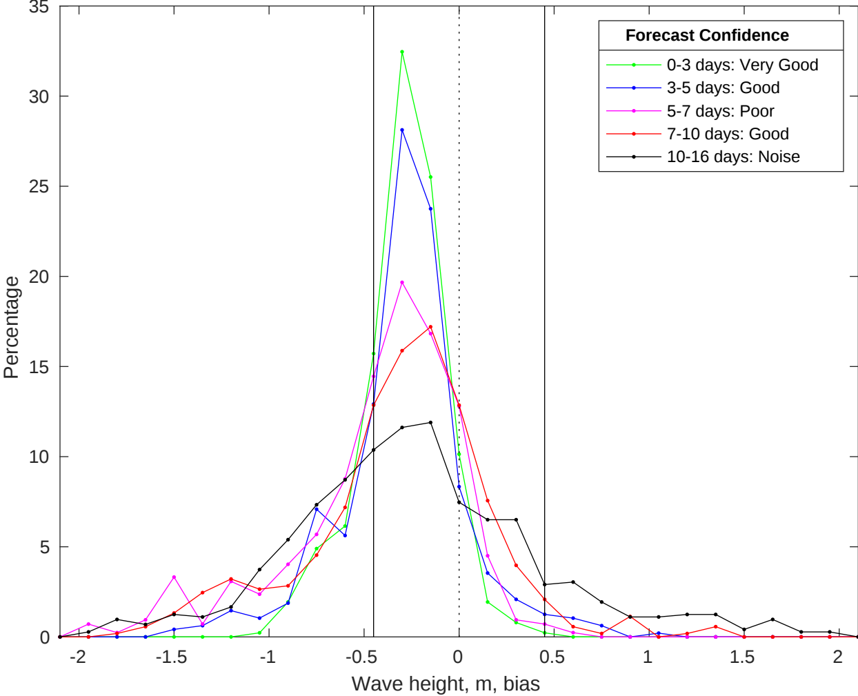
NDBC 42084 vs GFSWaves Bias Histogram: 20-Jan-2025
