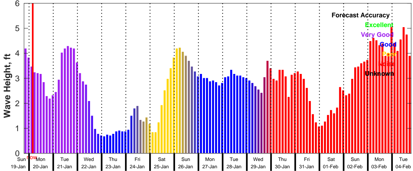
GFS Wave Forecast for NDBC 42084 from 19-Jan-2025 19:00:00 to 04-Feb-2025 19:00:00
