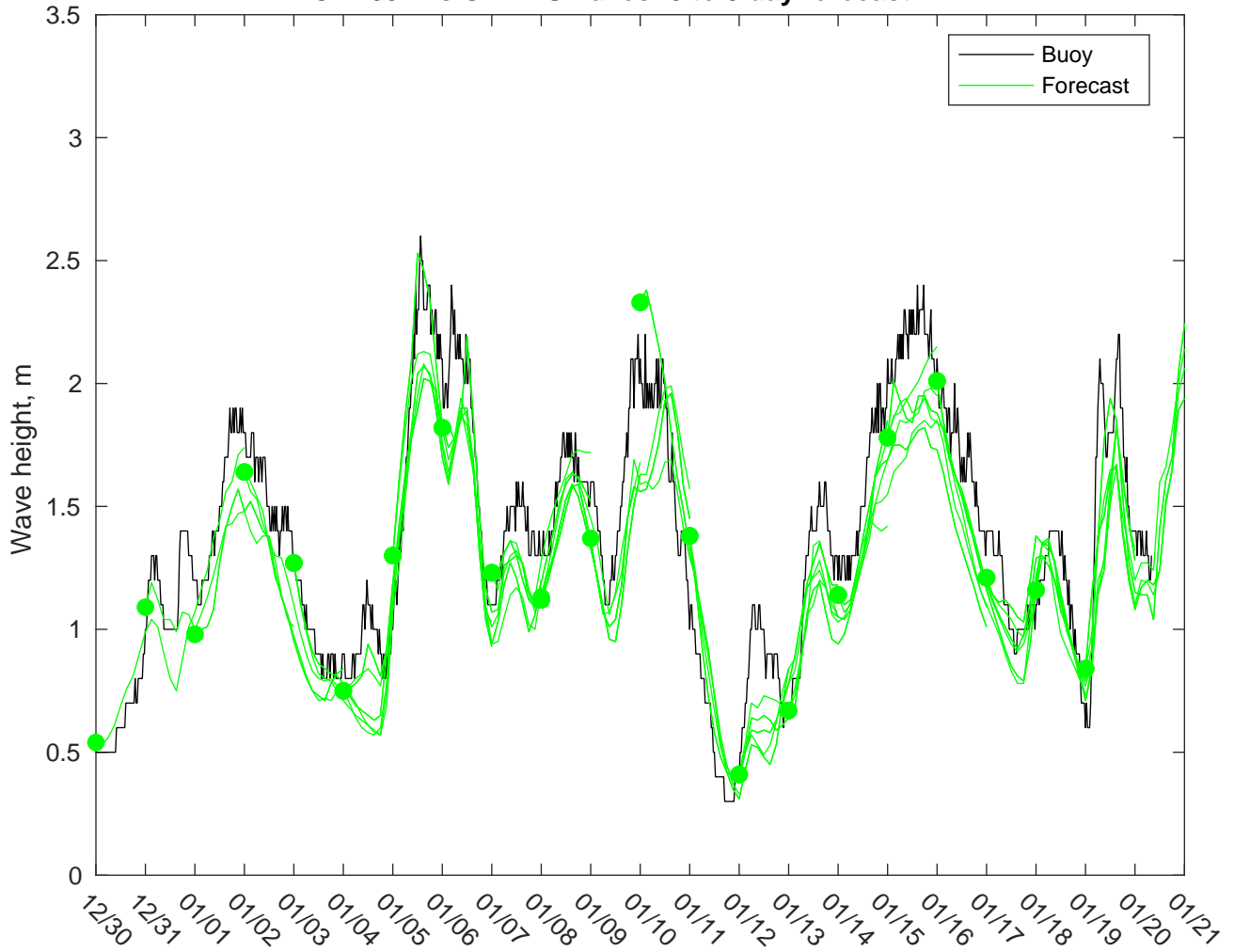
NDBC 42092 vs CMEMSWaves: 0 to 3 day forecast
