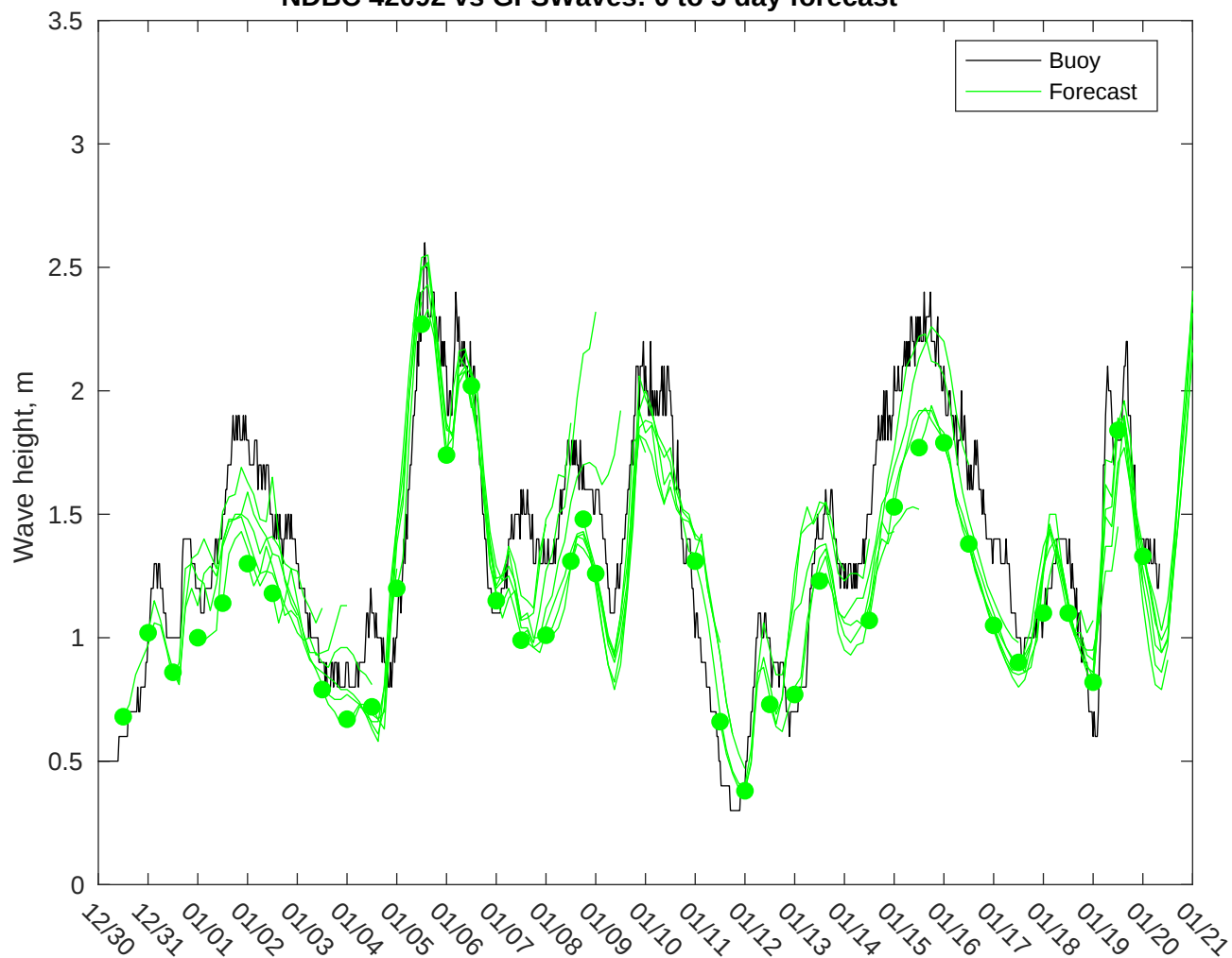
NDBC 42092 vs GFSWaves: 0 to 3 day forecast
