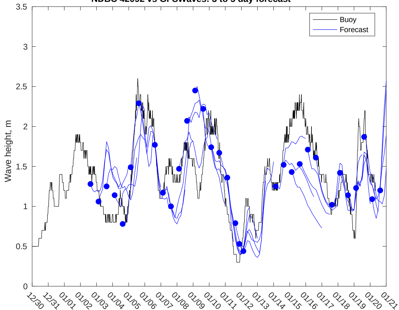
NDBC 42092 vs GFSWaves: 3 to 5 day forecast
