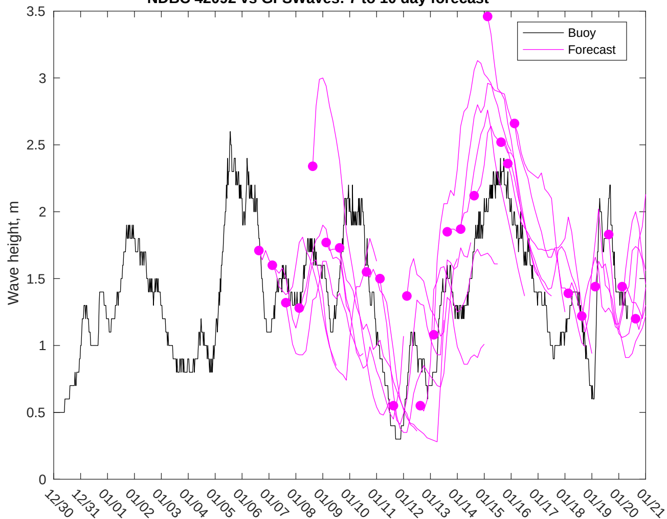
NDBC 42092 vs GFSWaves: 7 to 10 day forecast
