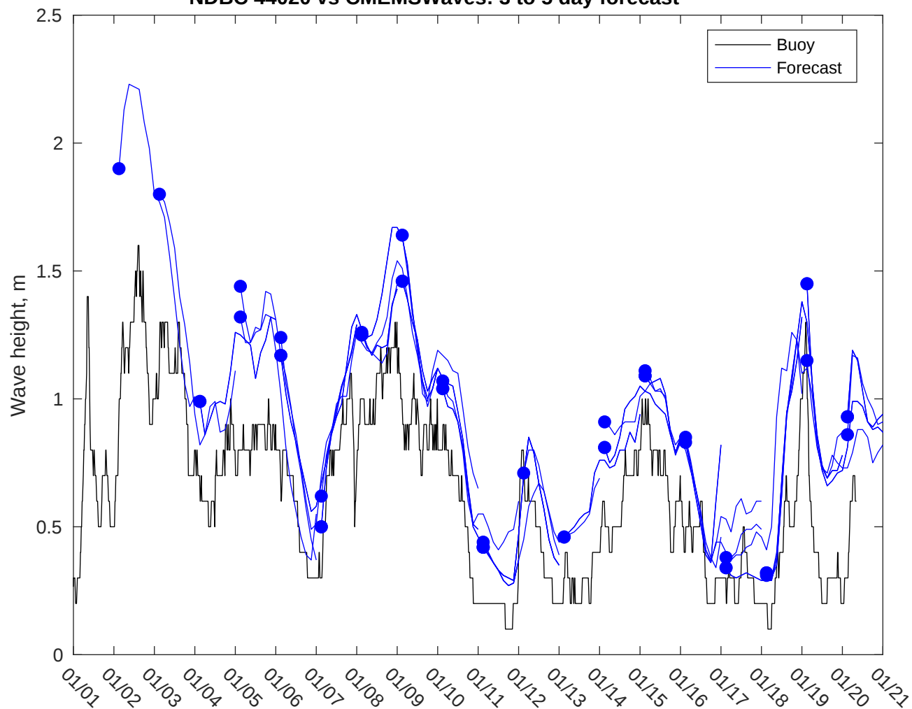
NDBC 44020 vs CMEMSWaves: 3 to 5 day forecast
