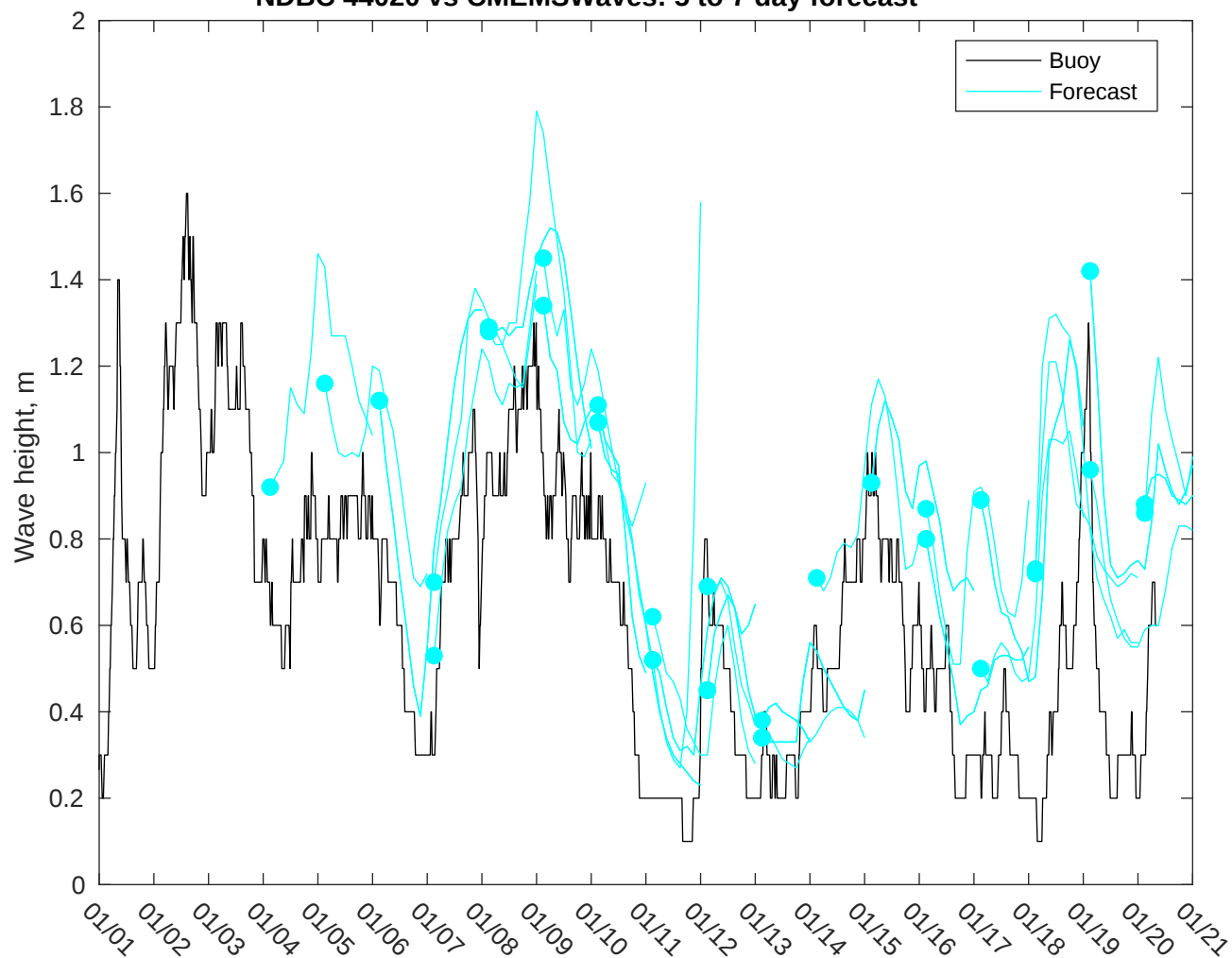
NDBC 44020 vs CMEMSWaves: 5 to 7 day forecast
