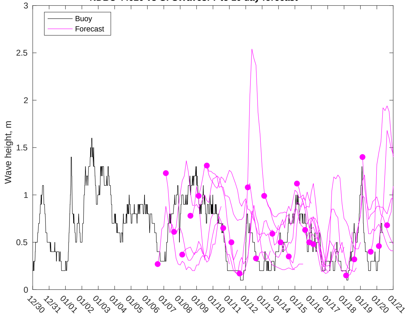
NDBC 44020 vs GFSWaves: 7 to 10 day forecast
