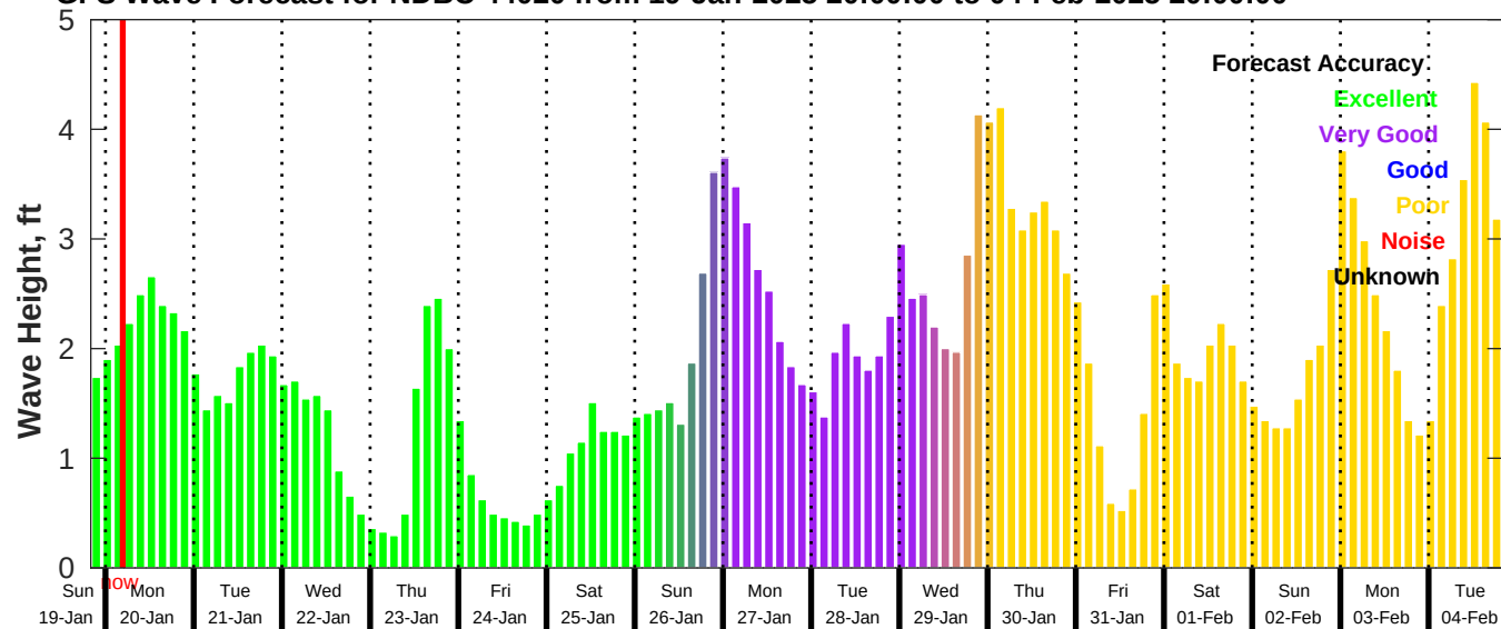
GFS Wave Forecast for NDBC 44020 from 19-Jan-2025 20:00:00 to 04-Feb-2025 20:00:00
