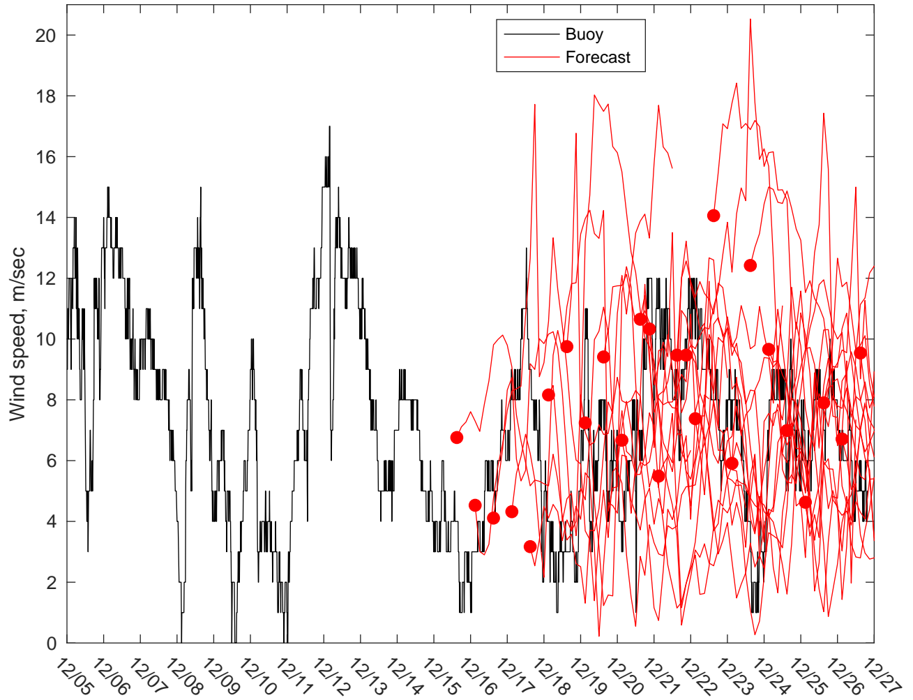
NDBC 44020 vs GFSWinds: 10 to 16 day forecast
