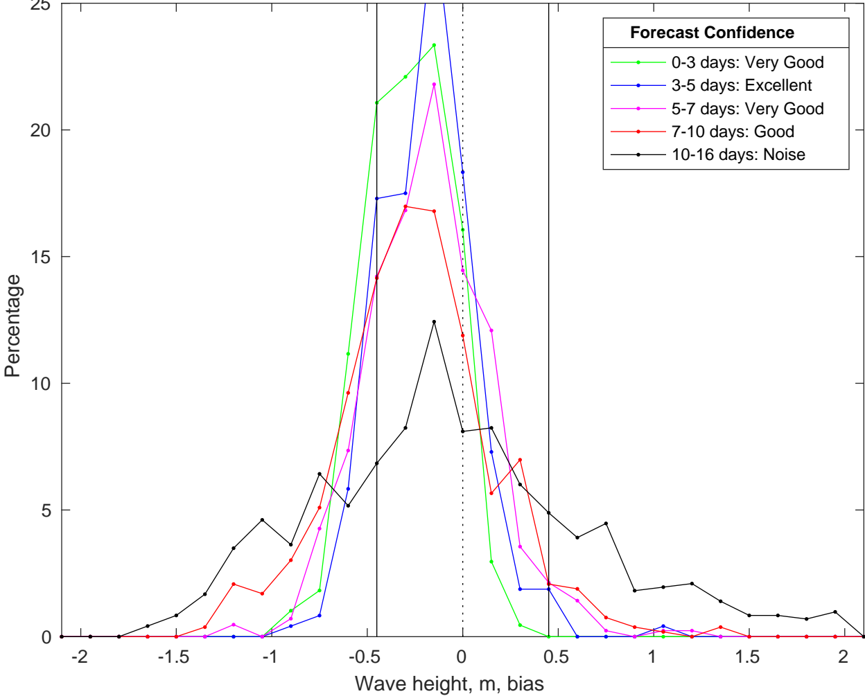
NDBC 46011 vs GFSWaves Bias Histogram: 20-Jan-2025
