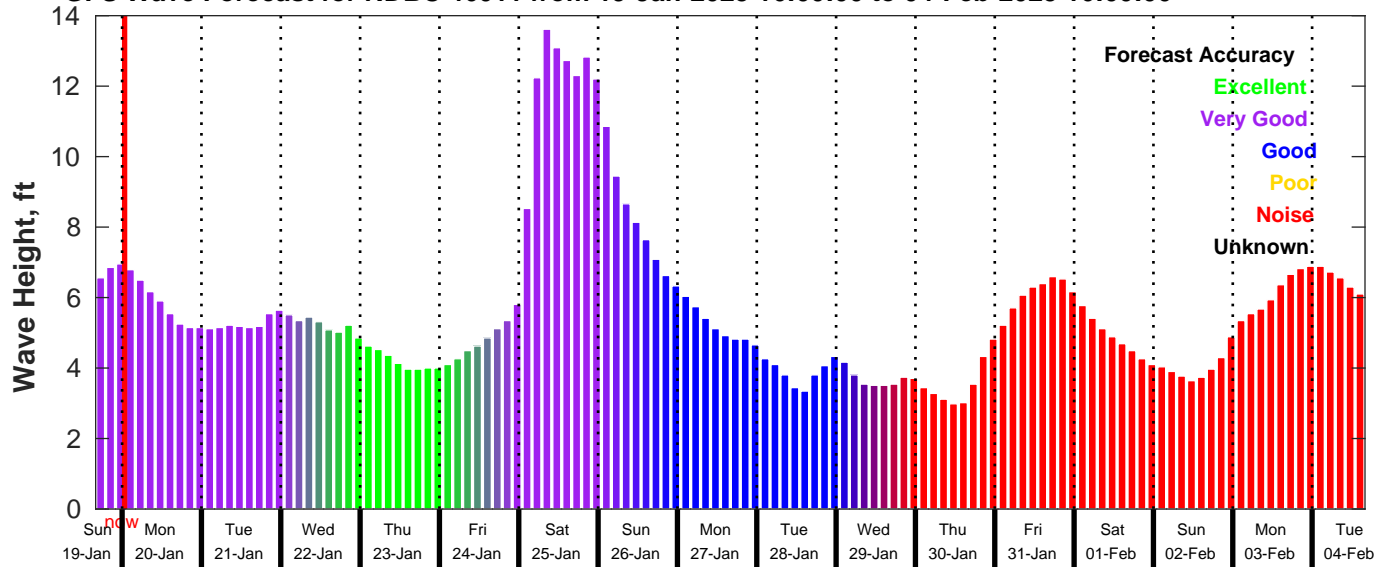
GFS Wave Forecast for NDBC 46011 from 19-Jan-2025 16:00:00 to 04-Feb-2025 16:00:00
