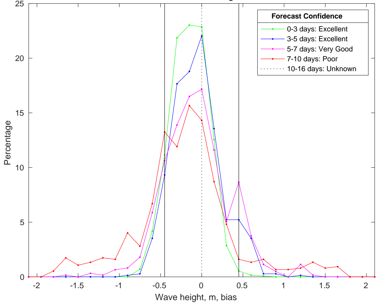
NDBC 46028 vs CMEMSWaves Bias Histogram: 20-Jan-2025
